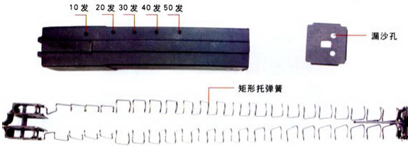
Four-row double-entry magazine
